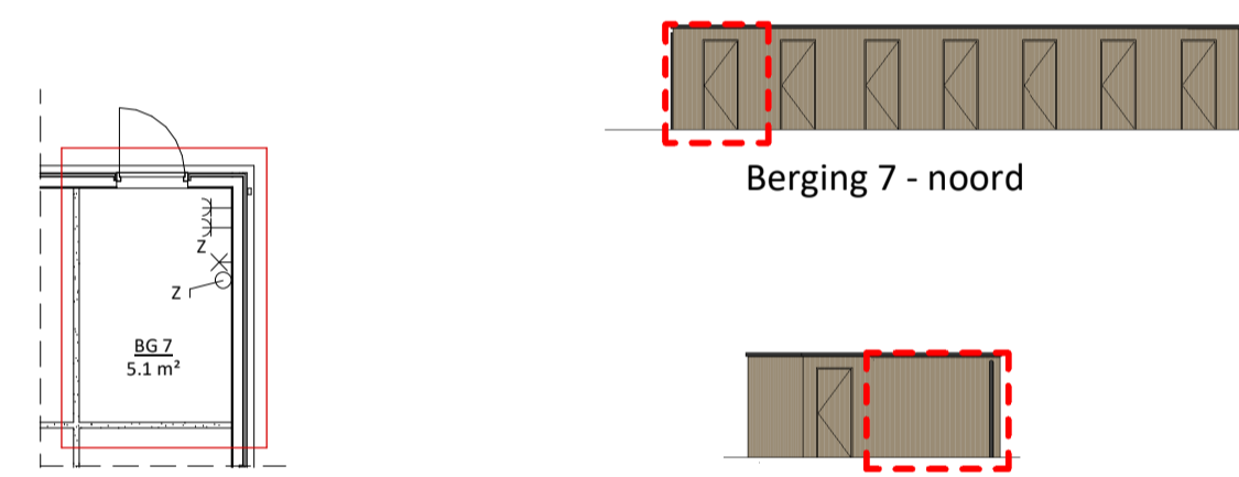
Berging - 1:100
